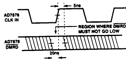
Figure 1. \overline{DMRD} Asynchronous Timing Constraint
