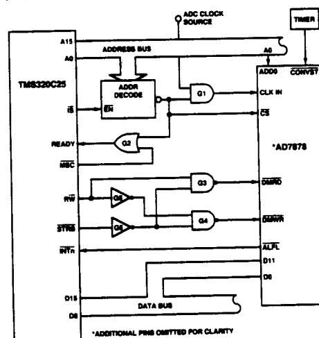
Figure 4. TMS320C25-AD7878 Asynchronous Clock Interface
