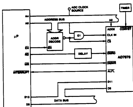
Figure 2. Asynchronous Clock Interfacing with the AD7878
