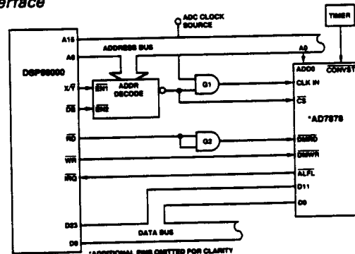
Figure 5. DSP56000-AD7878 Asynchronous Clock Interface
